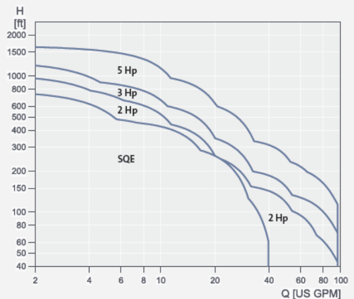
SmartFlo performance range: 0.5 to 5 Hp
